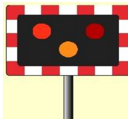
Flashing Red lights – STOP. Found at: Lifting Bridges, Level Crossings & Emergency Service Stations
